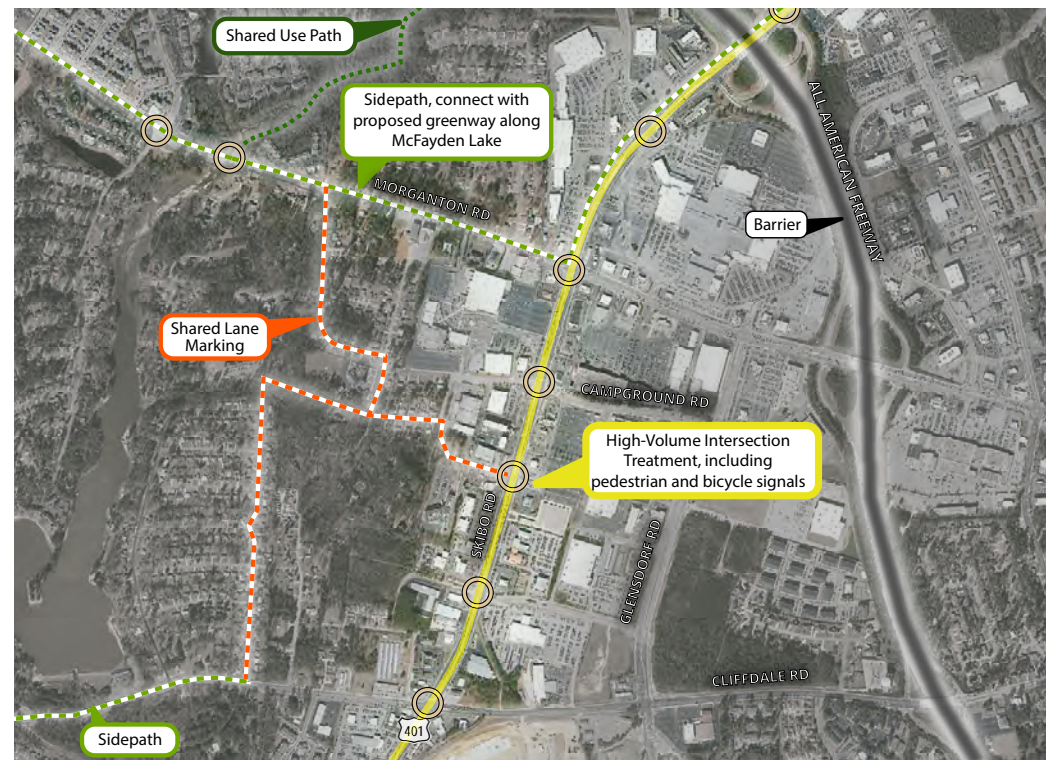
SKIBO ROAD HOT SPOT
