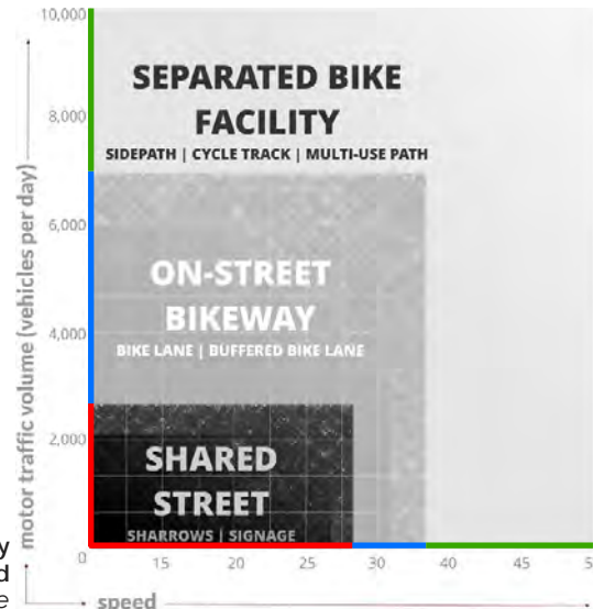
General Framework for Bikeway Selection by VPD and Speed Source: FHWA Bikeway Selection Guide
