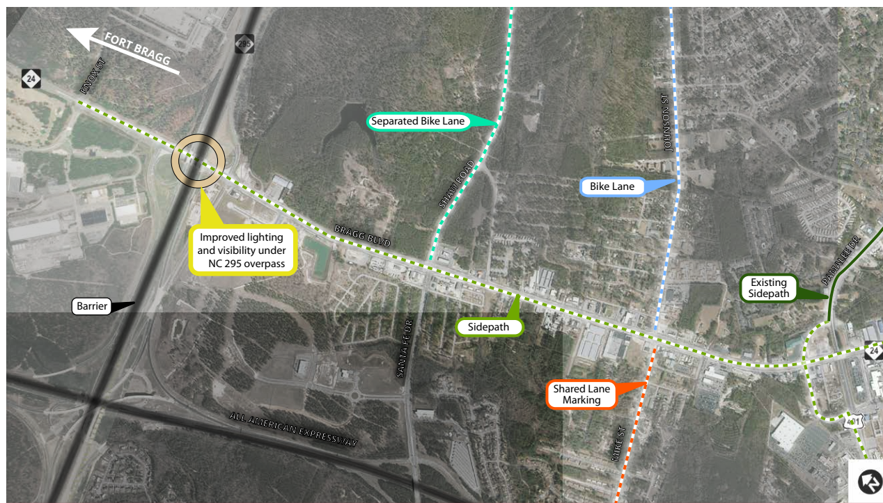
FIGURE 3.3: BRAGG BOULEVARD HOT SPOT
