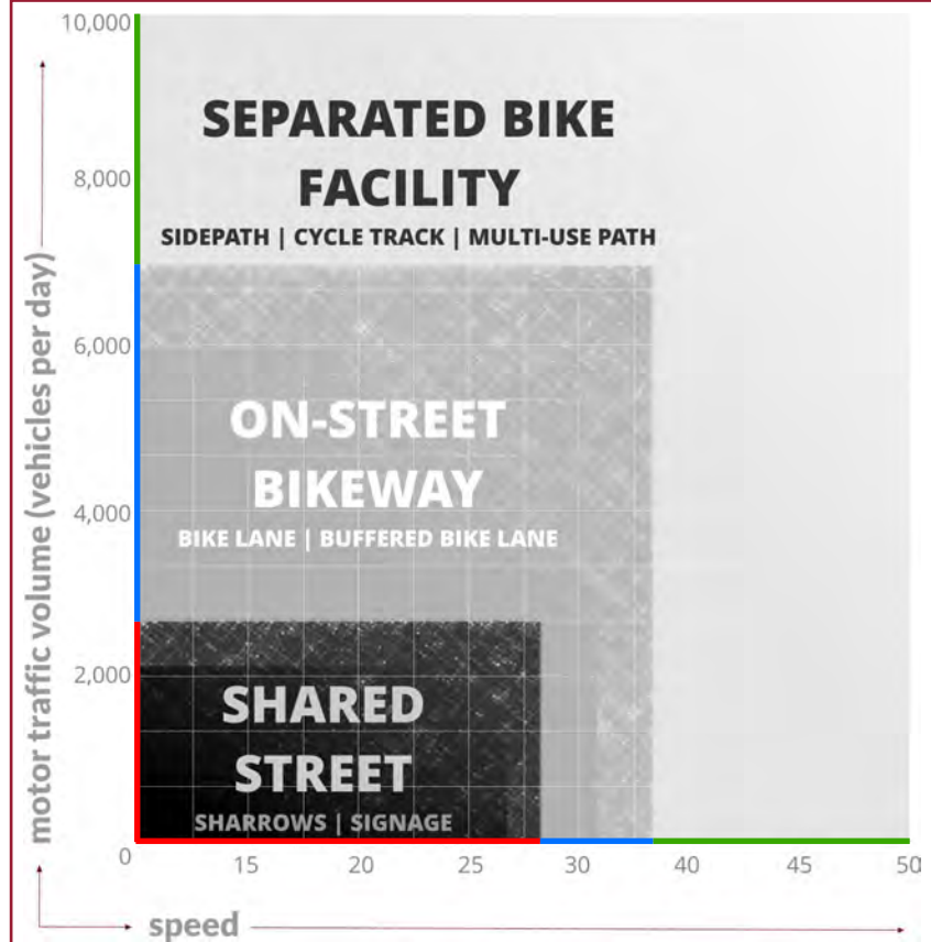
FIGURE 3.1: GENERAL FRAMEWORK FOR BIKEWAY SELECTION BY VPD AND SPEED Source: FHWA Bikeway Selection Guide
