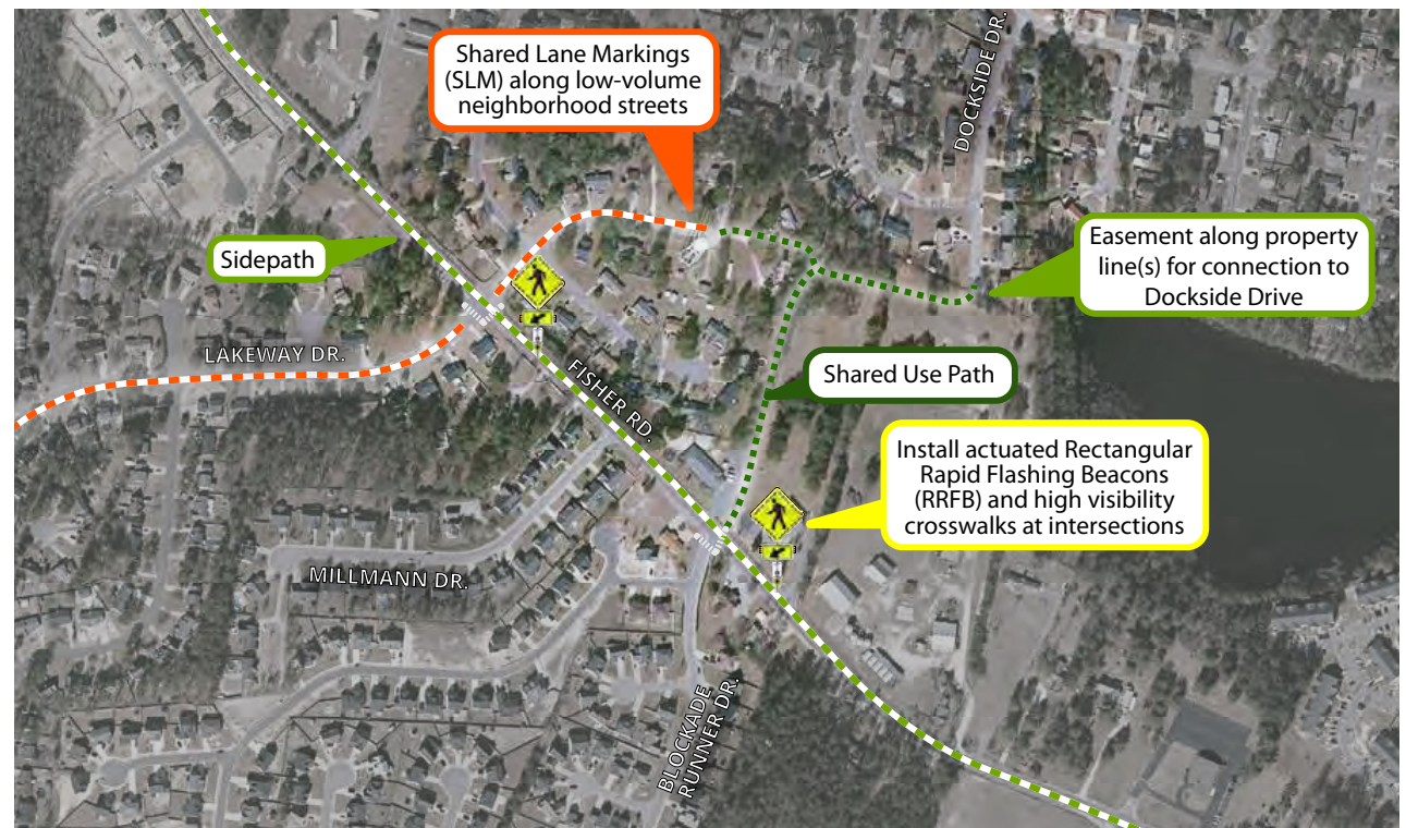
FIGURE 3.4: FISHER ROAD HOT SPOT
