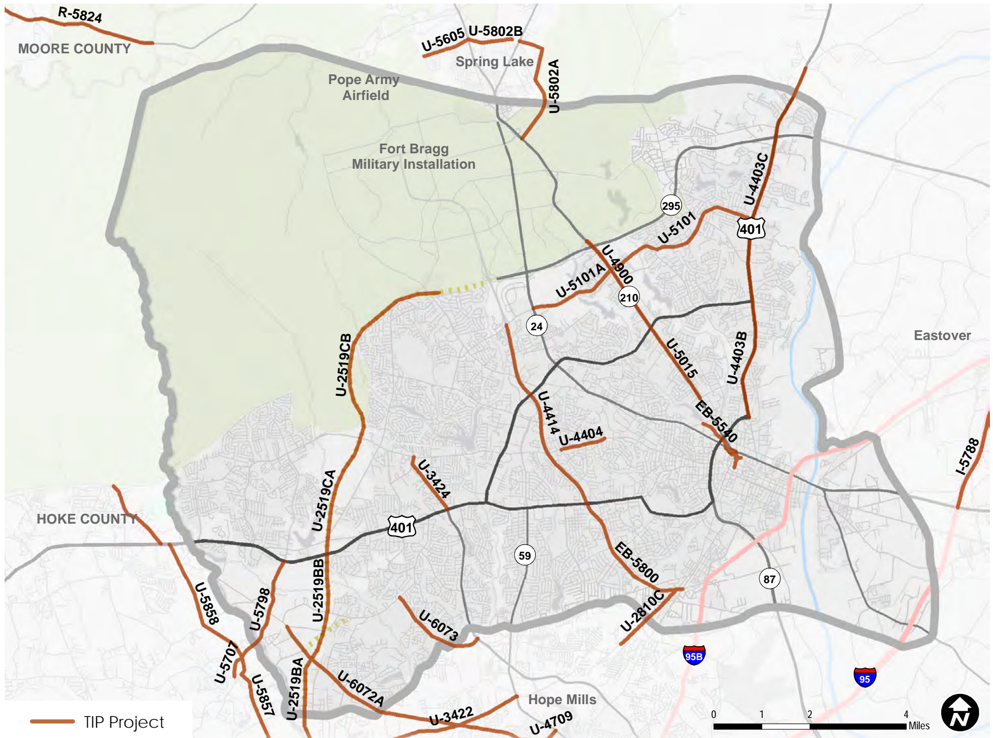
MAP 2.6: NCDOT PLANNED PROJECTS Source: NCDOT TIP 2018-2027
