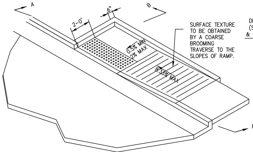
ISOMETRIC VIEW
